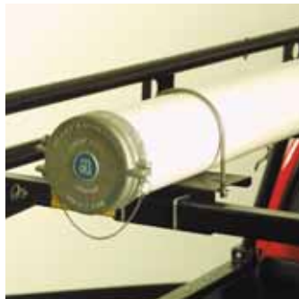
70-3 4" Diameter PVC Conduit Carrier Kit with Mounting Plate. Use with 4-1/2" O.D. PVC pipe schedule 40. PVC tubing not supplied.
