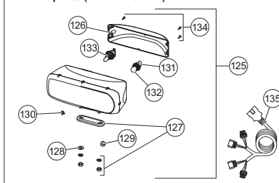
Headlamp Kits (2016 and earlier)
