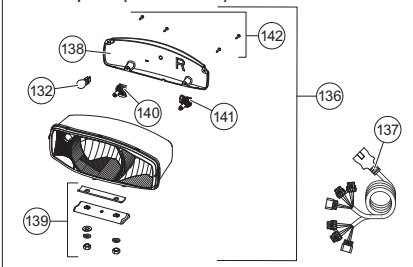
Headlamp Kits (2017 and later)
