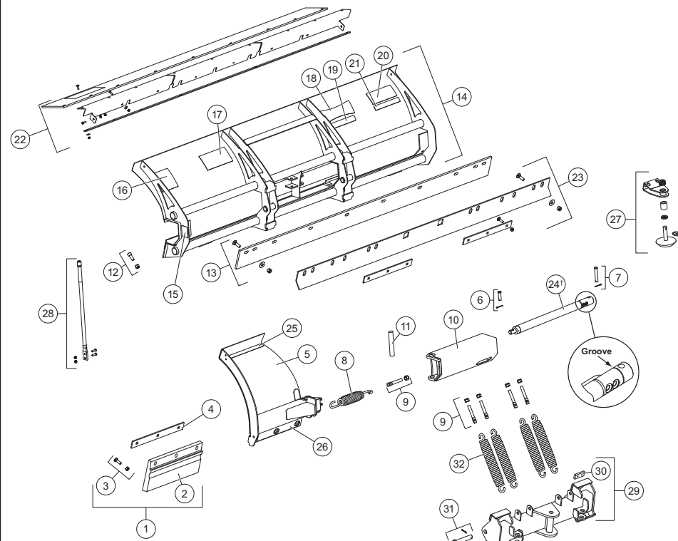
WIDE-OUT™ Blade Assembly 52810
